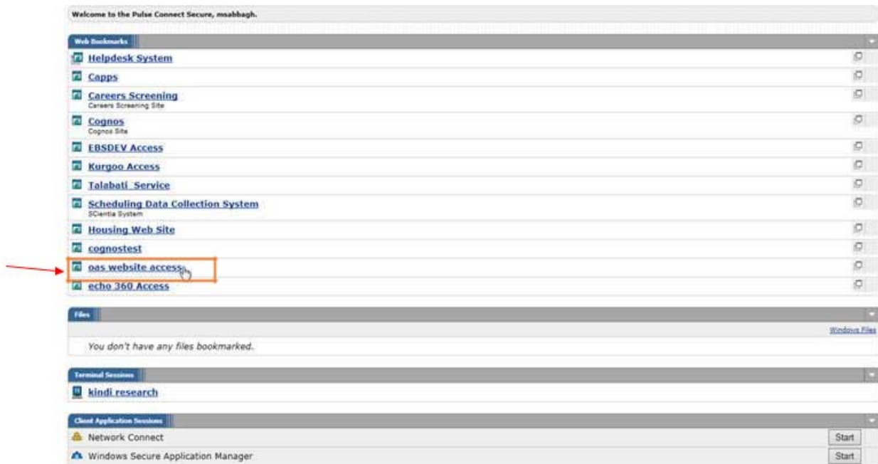
Figure 4: OAS access
